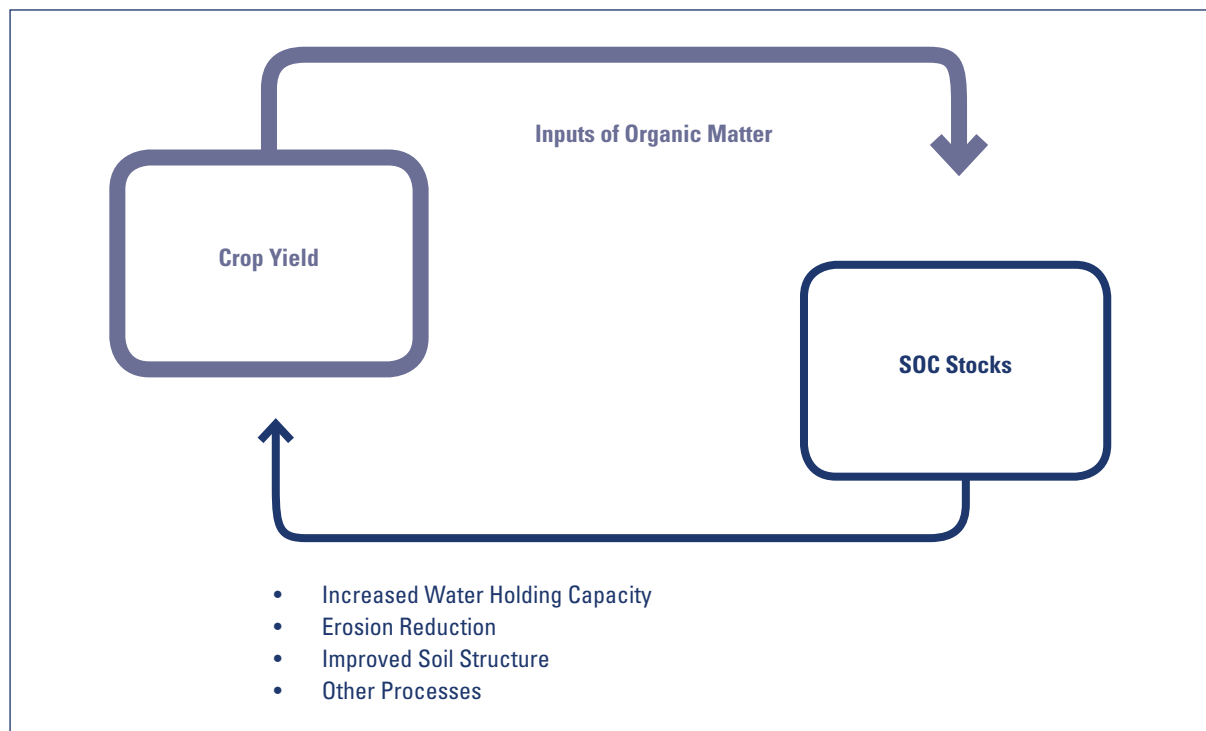
Figure 6. Coupling between SOC stocks and crop yield
