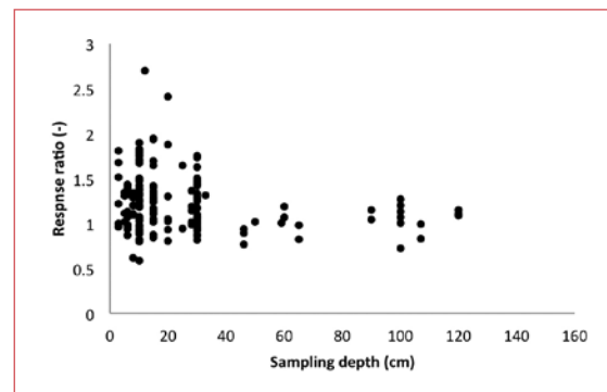
Figure 5. Response ratio (ratio of depth of integrated SOC stocks in alternatively managed or converted grassland to depth of integrated SOC stocks in traditionally managed grassland) vs. sampling depth (cm)
